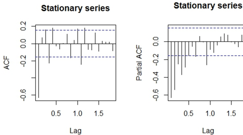
Figure 5. Correlogram of the stationary series.
