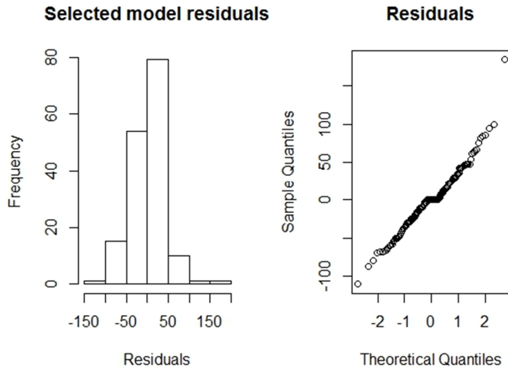
Figure 7. Distribution of the residuals of the selected model.
