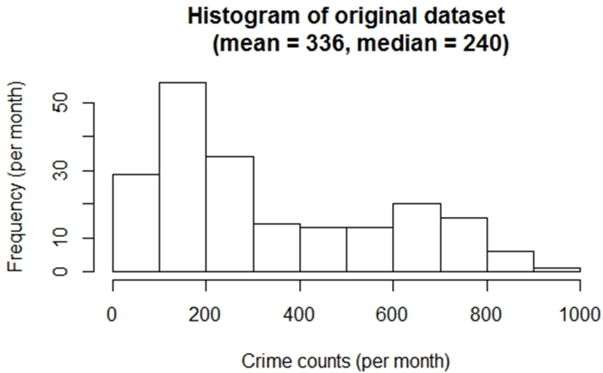
Figure 3. Histogram of original dataset.
